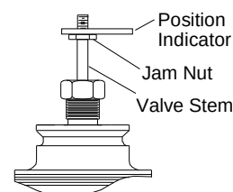
Figure 5: Installing Nut and Position Indicator
