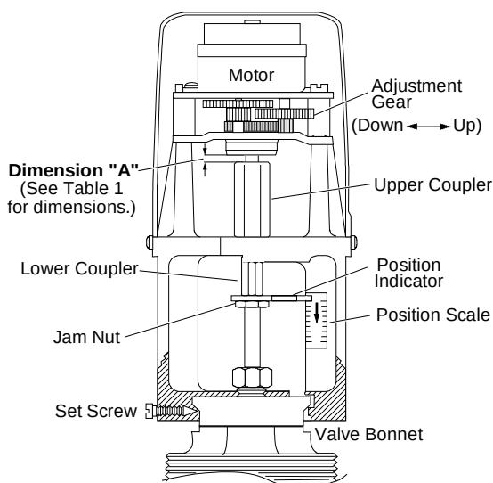
Figure 4: Actuator Components
