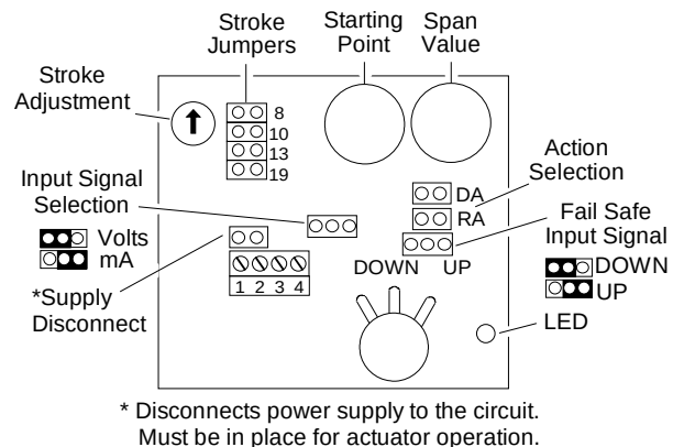
Figure 13: VA-7202 Components
